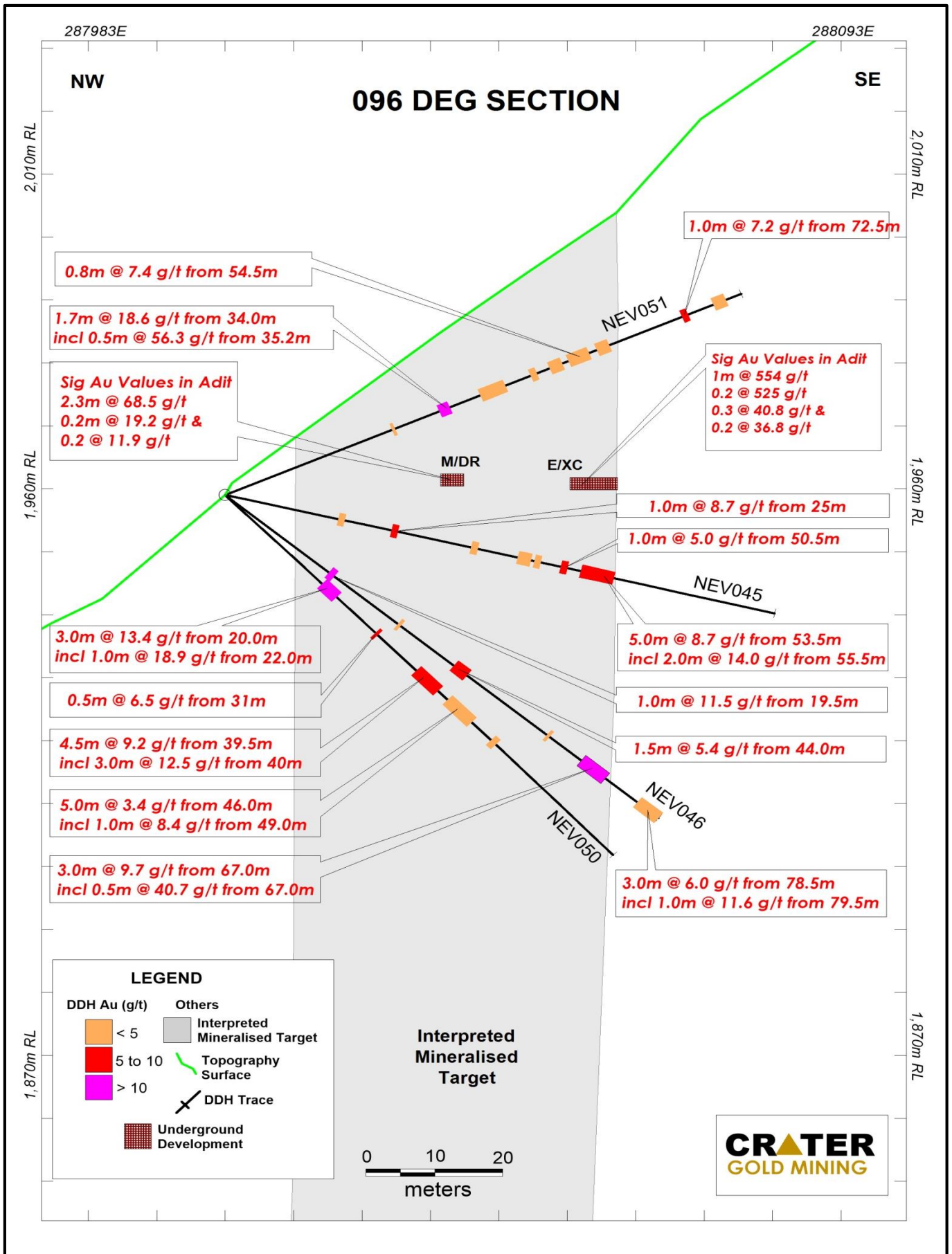
Figure 3 - Section of Drill Holes and Intercepts on 96° Bearing
