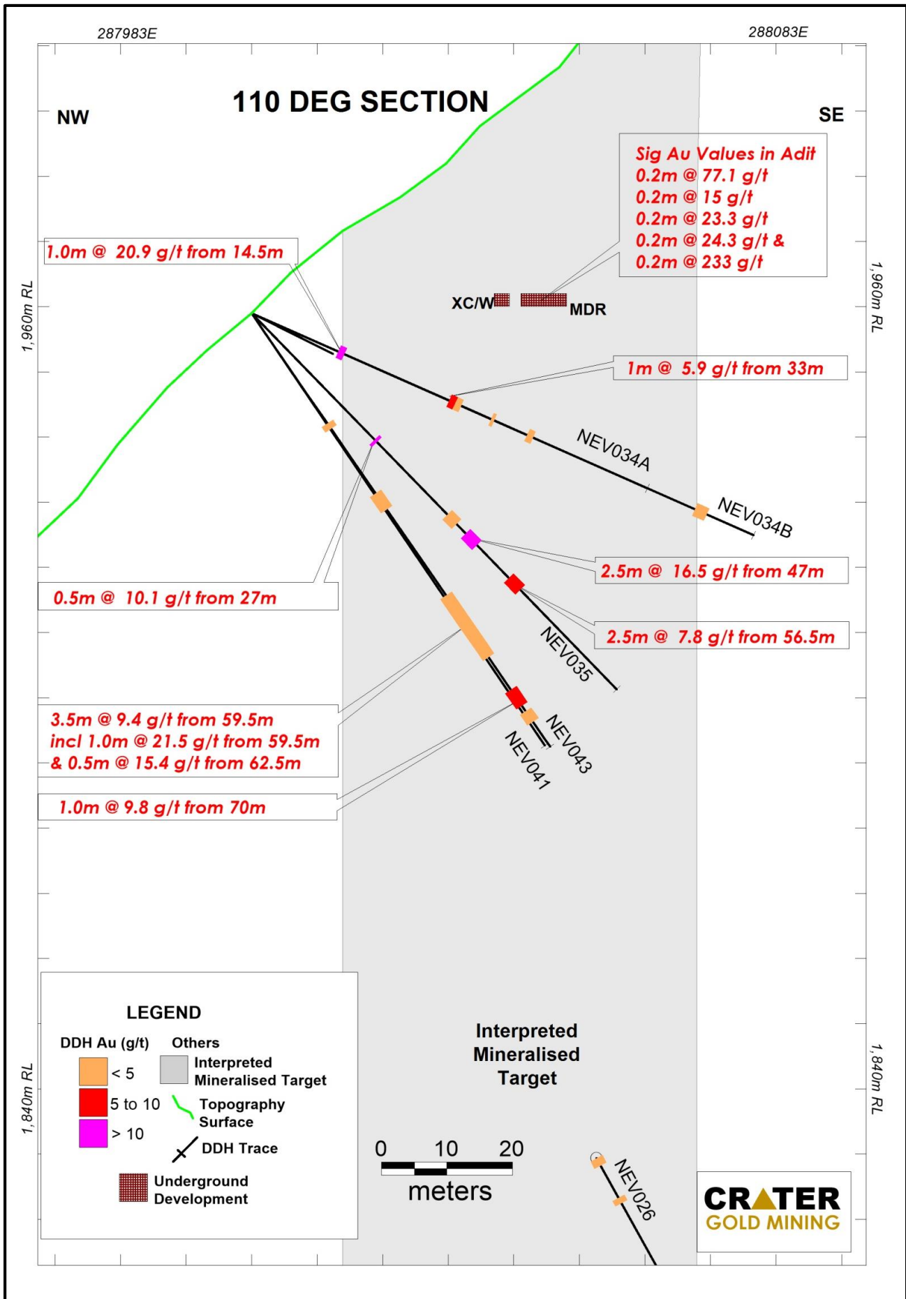
Figure 4 - Section of Drill Holes and Intercepts on 110° Bearing
