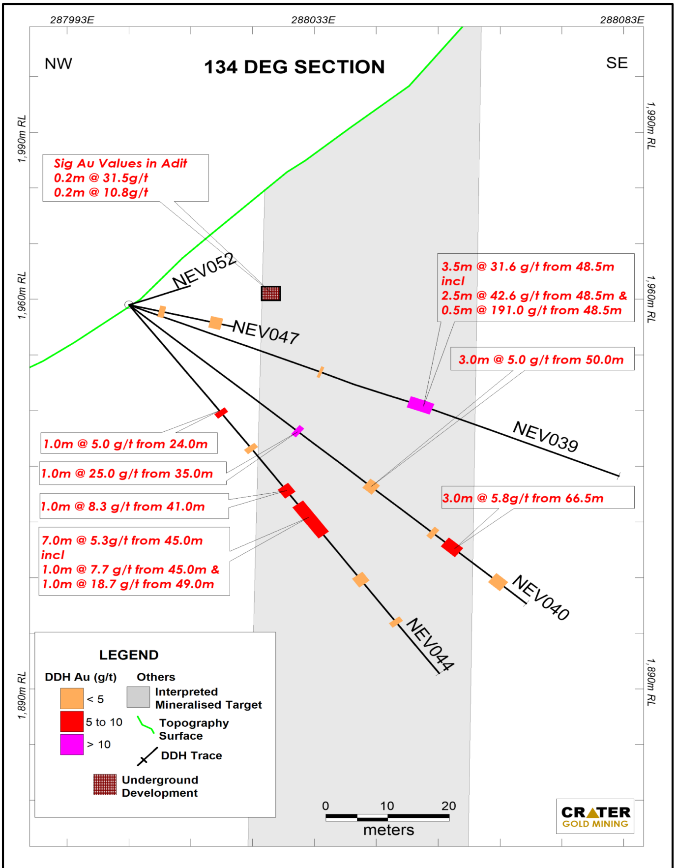
Figure 6 - Section of Drill Holes and Intercepts on 134° Bearing
